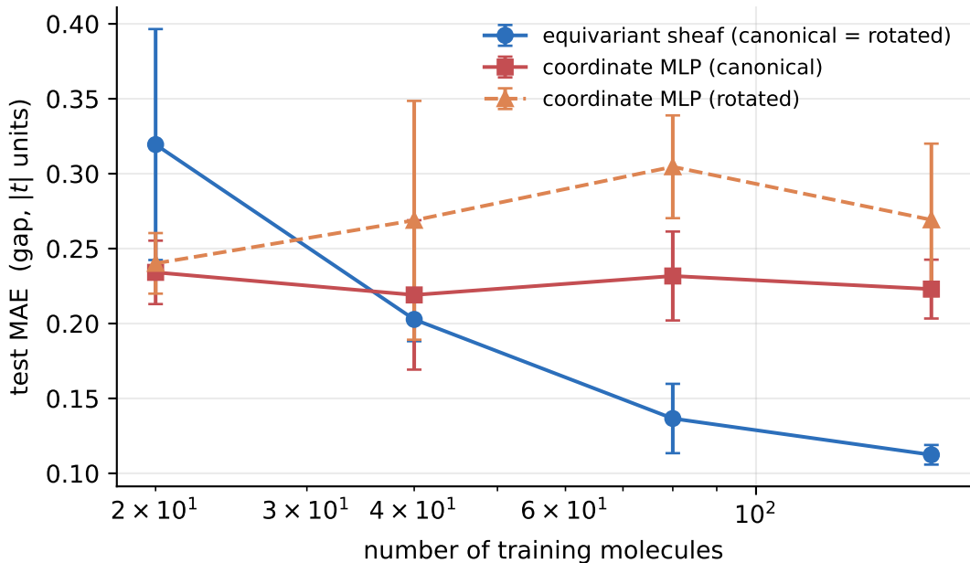
E4: equivariance gives lower error and rotation generalization
