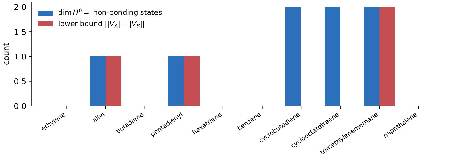
E2: sheaf cohomology counts non-bonding orbitals (alternant systems)
