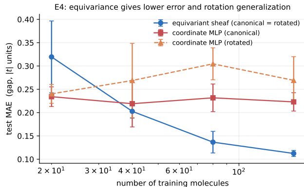
Fig. 3 E4: learning curves on the directional gap target. The equivariant sheaf model is more accurate and generalizes across orientations with no augmentation; the coordinate model plateaus and degrades on rotated test molecules.
