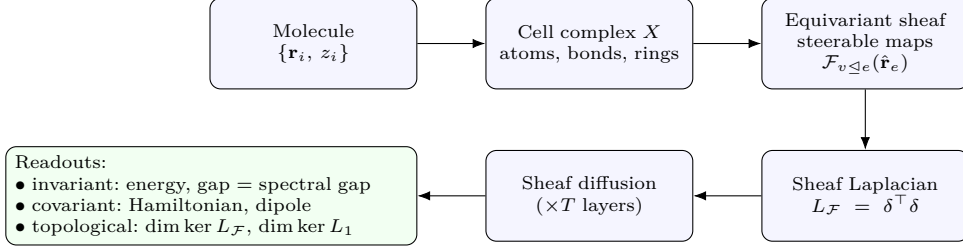
Fig. 1 Equivariant Cellular Sheaf Network (ECSN). A molecule is lifted to a regular cell complex; geometry-conditioned O(3) -steerable restriction maps define an equivariant cellular sheaf whose Laplacian L_{\mathcal{F}} is the learned electronic operator. Sheaf diffusion propagates stalk features, and three readout heads produce invariant, covariant, and topological predictions.
