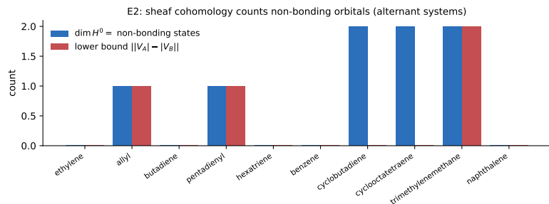
Fig. 2 E2: for the alternant systems, the computed cohomology dimension \dim H^0 (non-bonding orbital count) and the topological lower bound ||V_A| - |V_B|| of Cor. 4.8.
