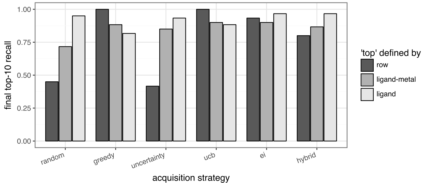
Top-k recall depends on how a 'top system' is defined
