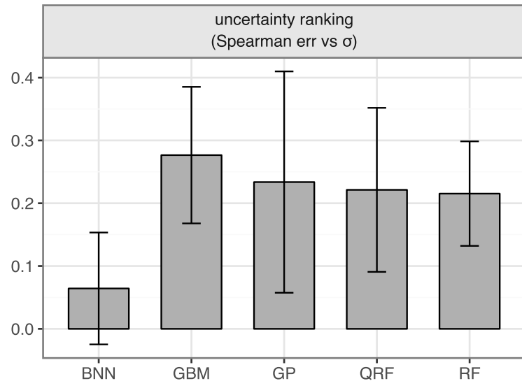
Uncertainty quality across estimators
