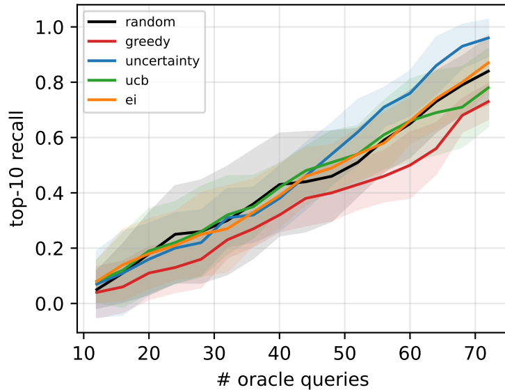
Top-10 recall vs budget
