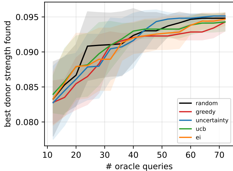
Best-found vs budget (pool=89)
