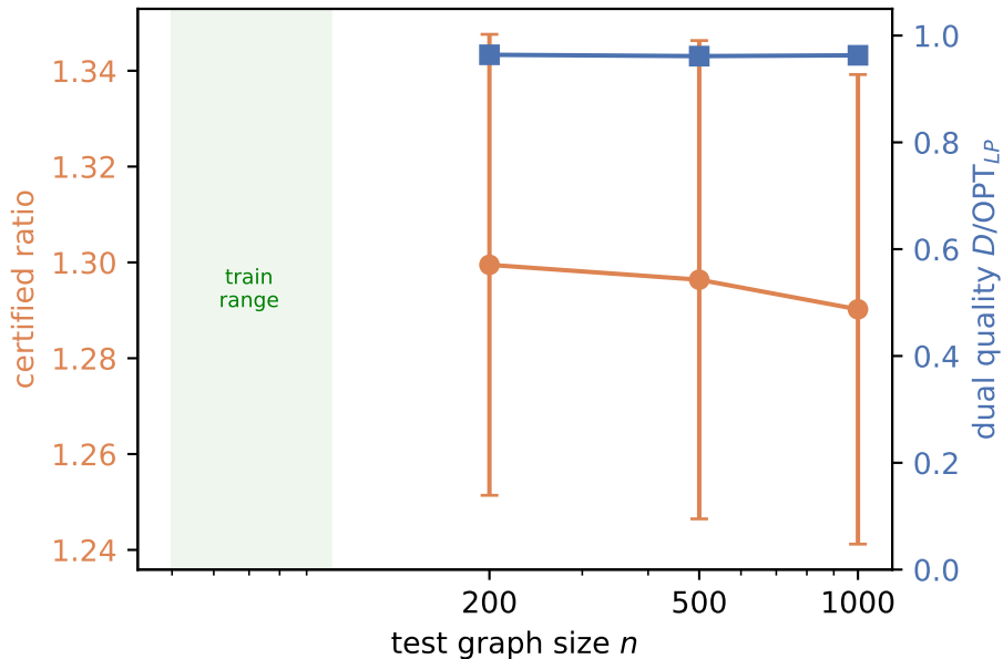
Extrapolation beyond training size
