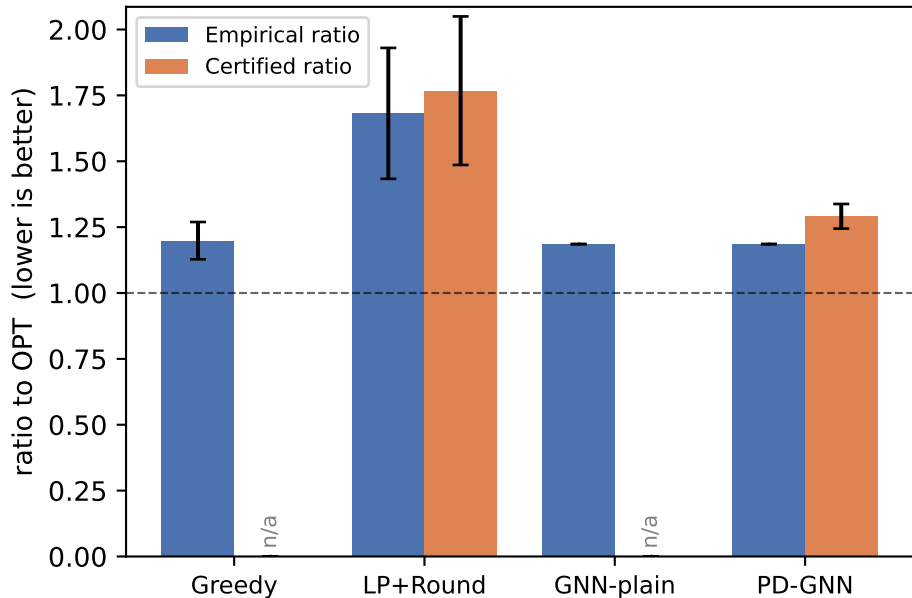
Vertex cover, G(n, p) , c = 5 , n \in [50, 100]
