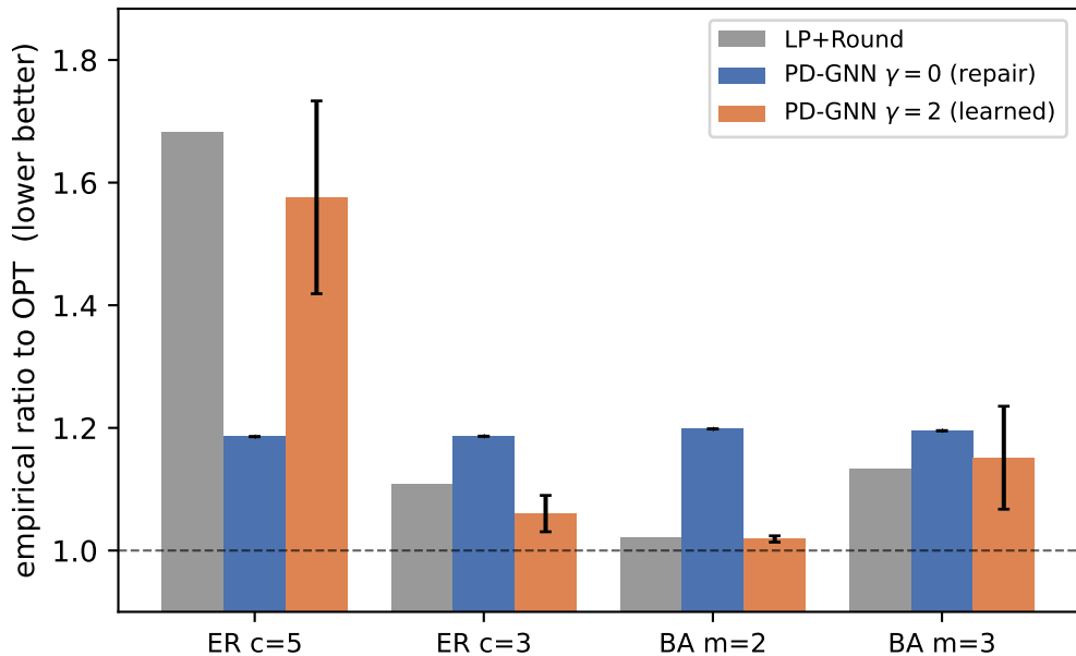
Coverage term: learned primal vs. repair
