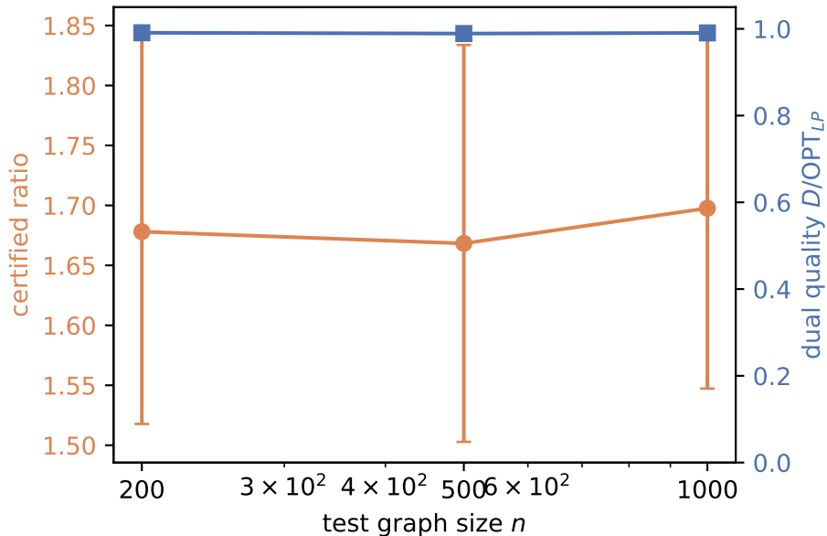
Extrapolation ( \gamma = 2 model)
