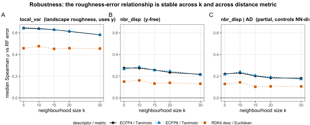
Figure 3: Stability of the roughness-error relationship across neighborhood size k and molecular distance metric. Median Spearman correlation over 30 targets between per-compound random-forest error and (left) a landscape roughness measure, (center) the activity-free neighborhood dispersion, and (right) the neighborhood dispersion after controlling for the applicability domain, for ECFP4/Tanimoto, ECFP6/Tanimoto, and a 12-descriptor Euclidean representation.
