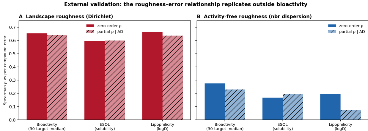
Figure 4: External validation on physicochemical regression benchmarks. Zero-order and applicability-domain-controlled (partial) Spearman correlations between roughness and per-compound error for (A) the landscape Dirichlet energy and (B) the activity-free neighborhood dispersion, for the 30-target bioactivity median and for aqueous solubility (ESOL) and lipophilicity (logD).
