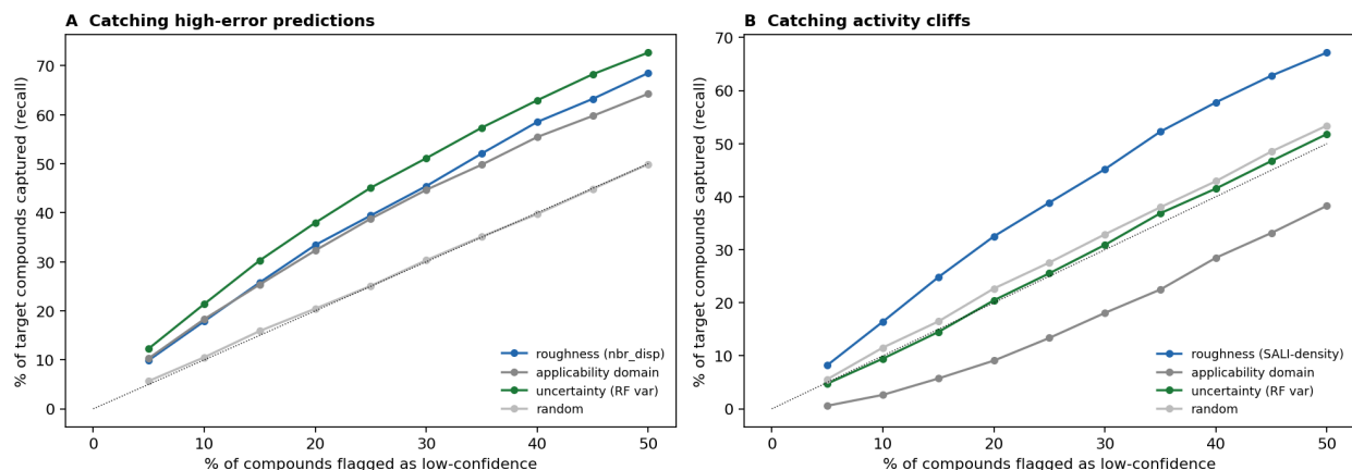
Figure 2. Operational triage value of a structure-only roughness flag. Fraction of (A) high-error predictions (top-quartile per-compound error) and (B) labeled activity cliffs recovered as a function of the percentage of compounds flagged as low-confidence, averaged over 30 targets, ranking by roughness (blue), the applicability domain in its standard orientation (gray), random-forest tree variance (green), or at random (dotted).
