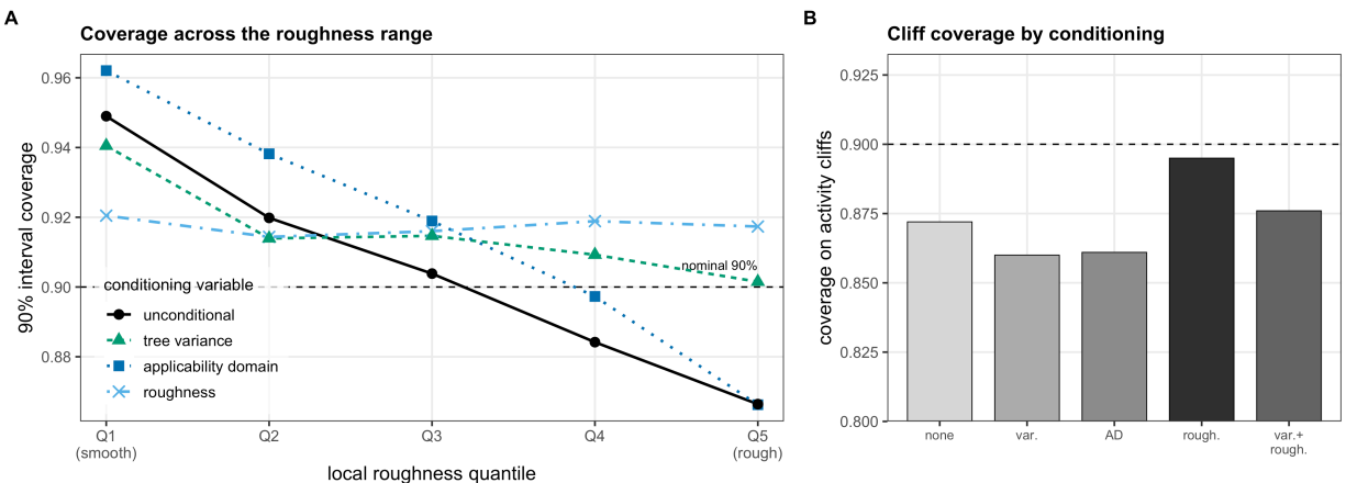
Figure 6: Roughness is the per-compound scale for cliff-valid conformal intervals. (A) Coverage of 90% inductive-conformal intervals as a function of local-roughness quantile (Q1 smoothest to Q5 roughest), for unconditional intervals and Mondrian intervals conditioned on random-forest tree variance, the applicability domain, or the activity-free roughness (dashed line, nominal). Unconditional, variance-, and applicability-domain-conditioned coverage all fall with roughness; only roughness conditioning holds it flat. (B) Coverage on labeled activity cliffs for the same conditionings and for the combined variance-plus-roughness score. Variance and applicability-domain conditioning leave cliff coverage at or below the unconditional level; roughness restores it toward nominal. Median over 30 targets and 50 calibration/evaluation splits.
