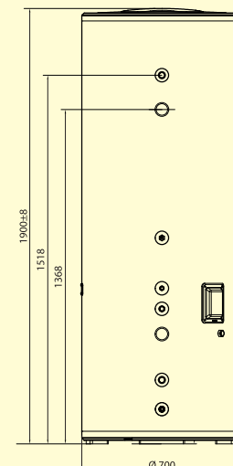
Tank 4 - 500 L
