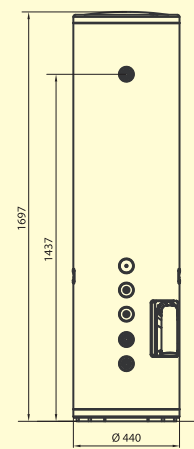
Tank 1 - 150 L
