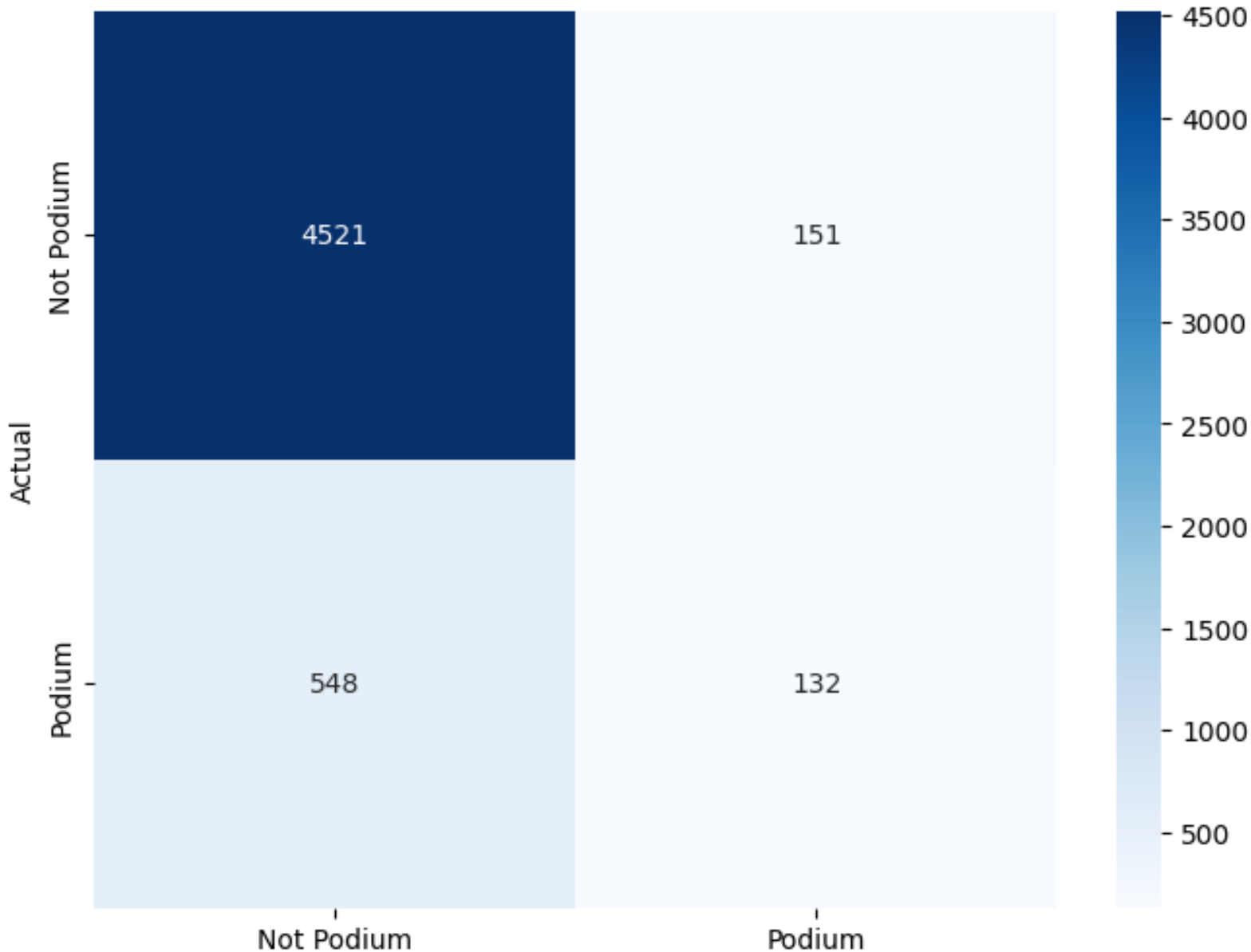
Confusion Matrix
