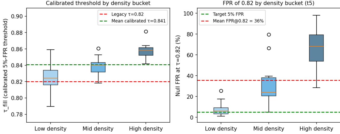
Figure 1: Calibrated threshold by density bucket (left) and null FPR at 0.82 (right). The fixed threshold 0.82 has 35.7% average null FPR, reaching 99% in high-density anchor cells. Calibrated \tau_{\text{fill}} \approx 0.841 is stable across all splits.
