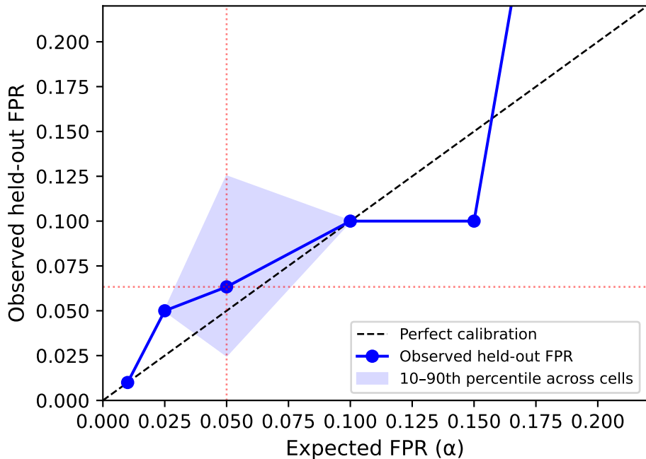
Figure 6: Null Calibration Curve Points near diagonal \rightarrow calibration valid
