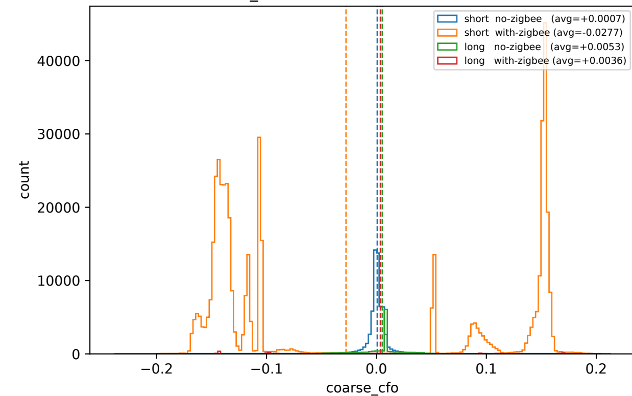
coarse_cfo distribution (dashed = mean)
