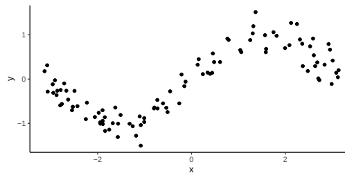
Figure 24: A simulated sine wave dataset, used to evaluate overfitting.
