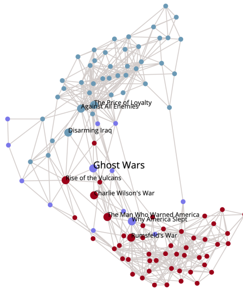
Figure 17: An example solution to [Interactive Political Books] part (c). The currently selected book is Ghost Wars. All its neighbors are also labeled, but in a smaller font.
