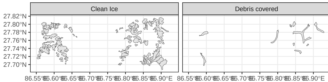
Figure 12: An example result for Himalayan Glaciers (a).
