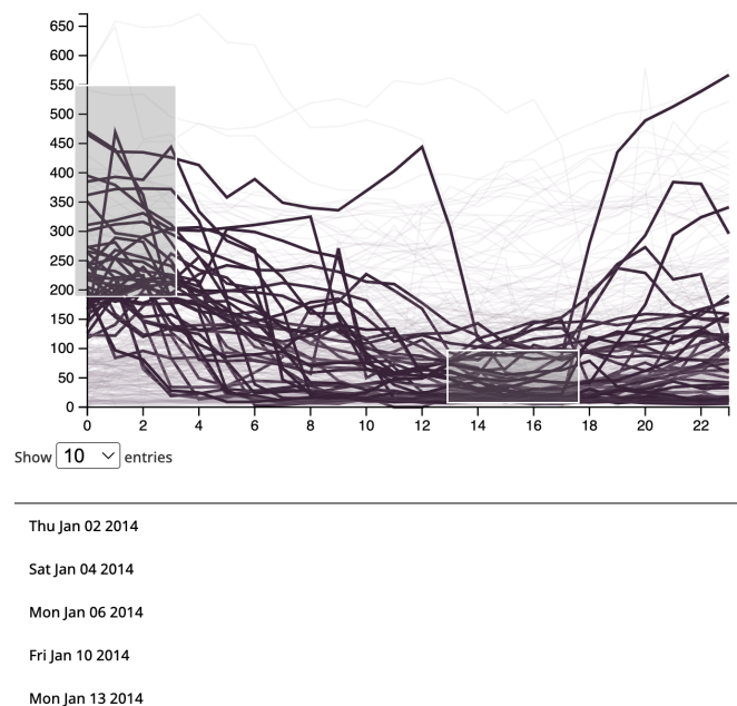
Figure 11: An example solution to [Air Pollution Time Searcher].
