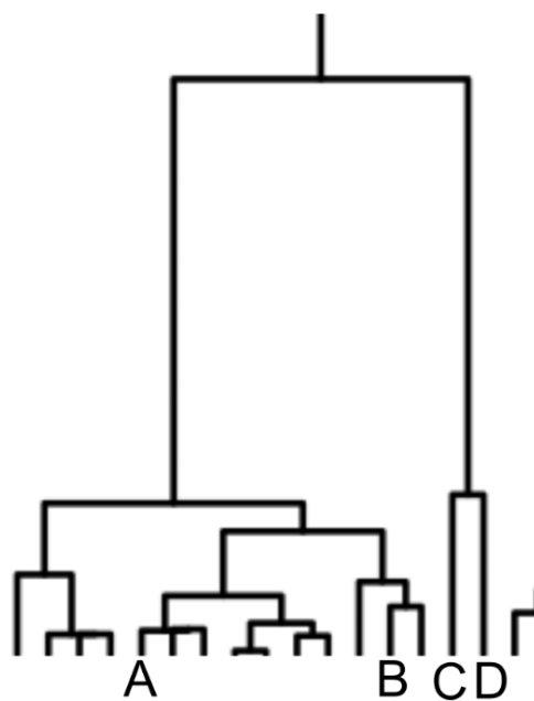
Figure 20: A subset of a large hierarchical clustering tree
