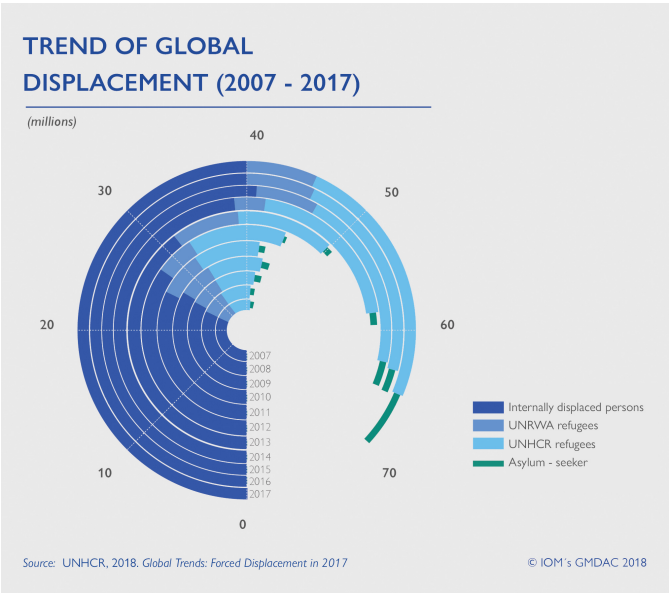
Figure 2: Patterns of displacement, from the Migration Data Portal.
