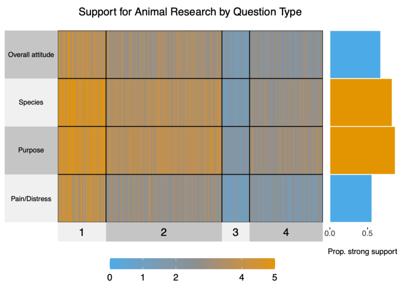
Figure 21: Responses from Sandgren and Streiffer (2022).
