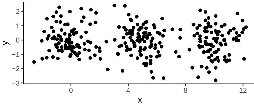
Figure 23: An example simulated dataset from problem 2.
