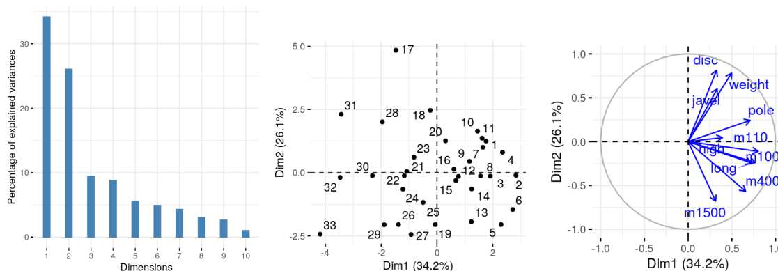
Figure 22: The PCA of the decathlon data, from Chapter 7 of Holmes and Huber's Modern Statistics for Modern Biology.
