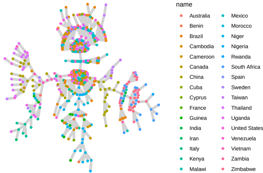
Figure 15: Example output created by [Improving Initial Visualizations] part (b). There are too many colors in this plot.
