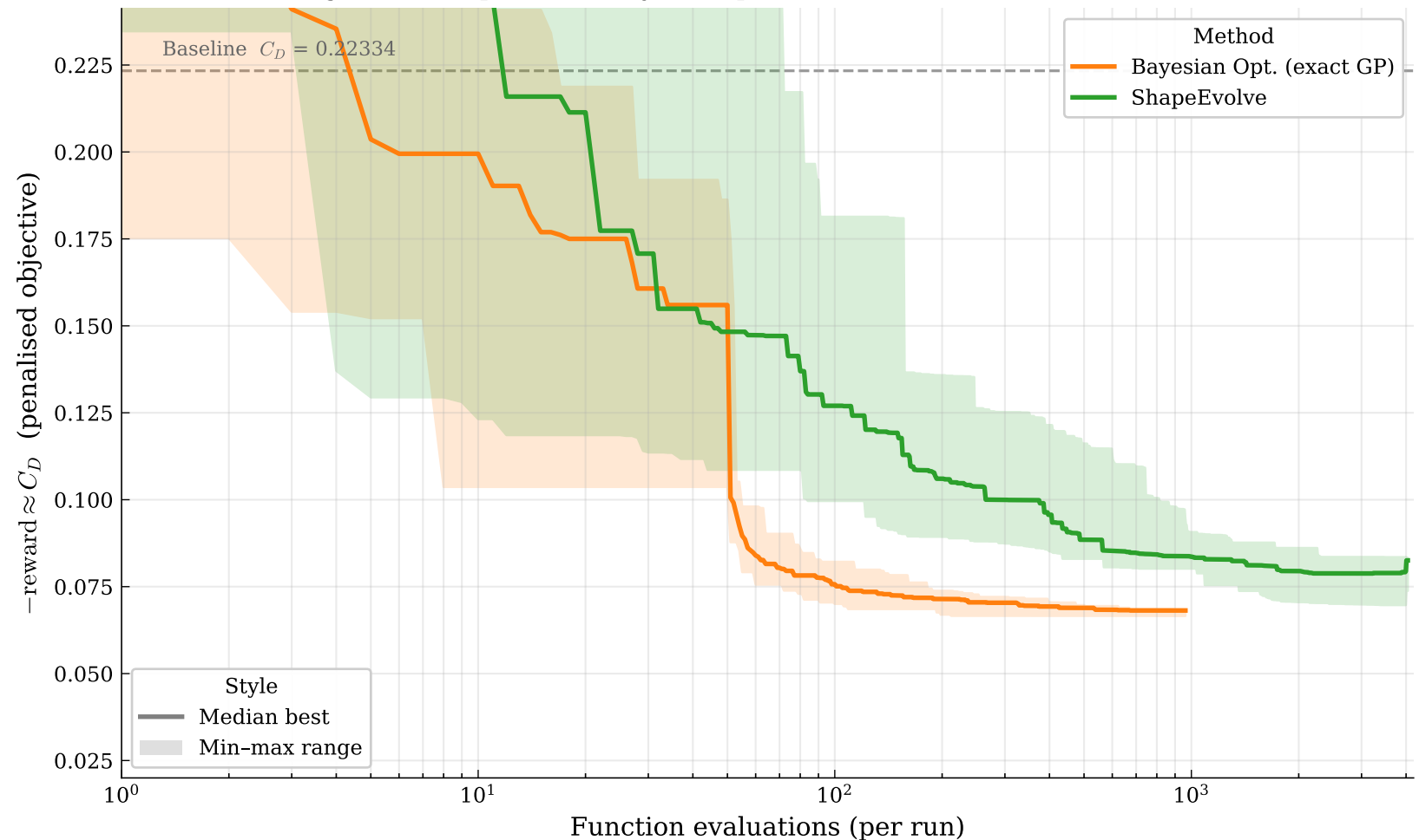
DrivAer* (Estate, vtk_E) — C_D -constrained ( C_l \leq -0.10 ) optimisation Convergence: best penalised objective per run (solid = median, band = min-max)
