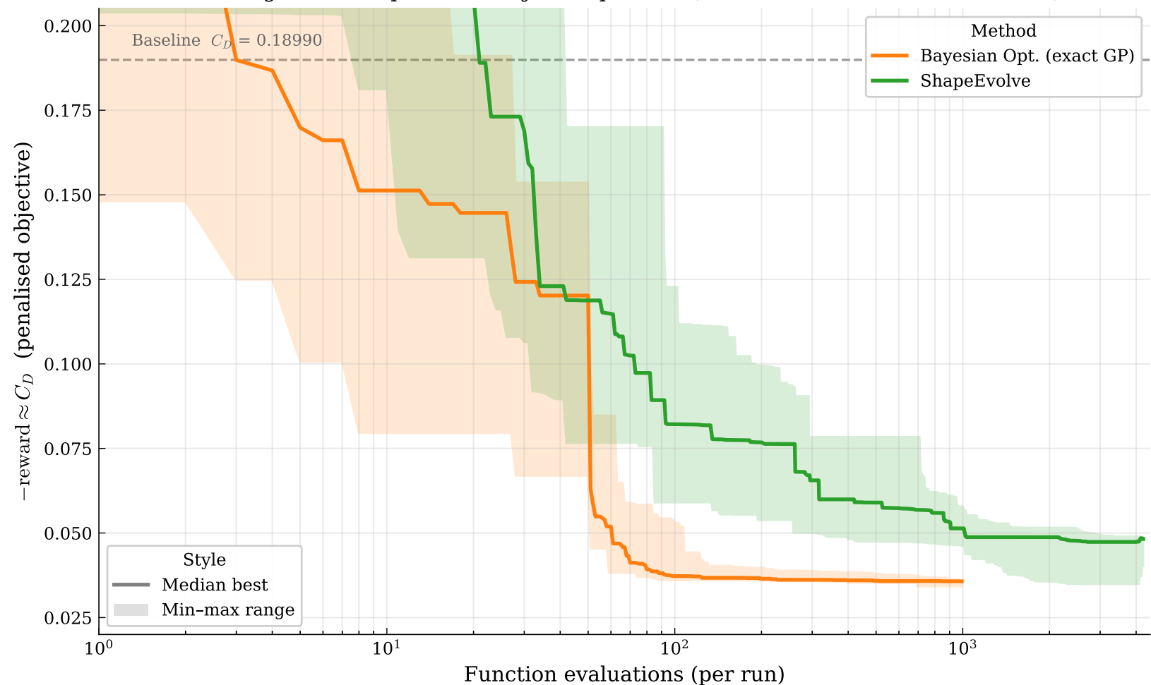
DrivAer* (Fastback, vtk F) — C_D -constrained ( C_l \leq -0.10 ) optimisation Convergence: best penalised objective per run (solid = median, band = min-max)
