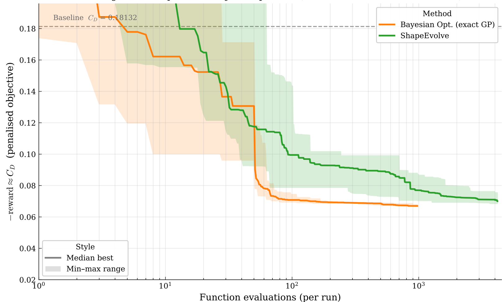
DrivAer * (Notchback, vtk N) — C_D -constrained ( C_l \leq -0.10 ) optimisation Convergence: best penalised objective per run (solid = median, band = min-max)
