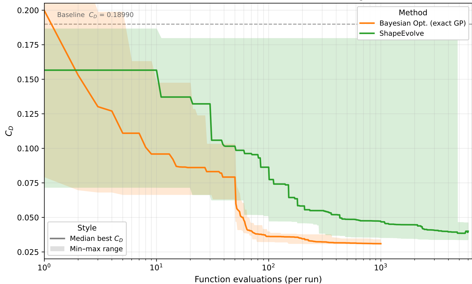
DrivAer Star (Fastback, vtk_F) — Convergence: best C_D vs function evaluations (solid = median across runs, band = min-max range)
