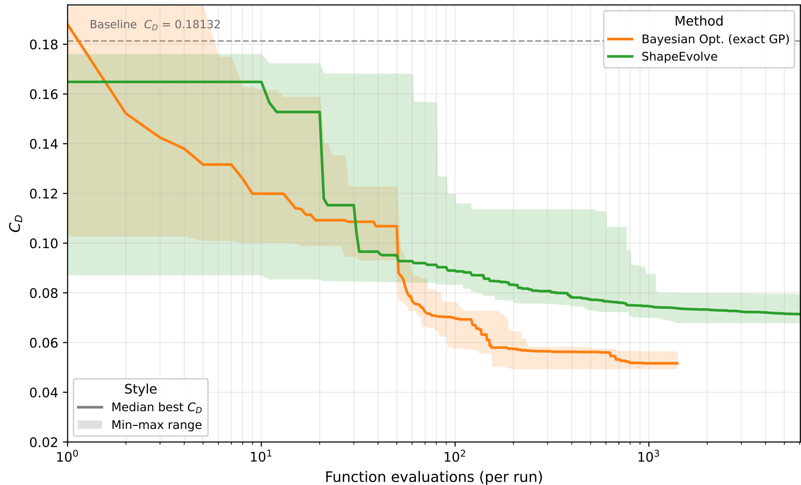
DrivAer Star (Notchback, vtk_N) — Convergence: best C_D vs function evaluations (solid = median across runs, band = min-max range)
