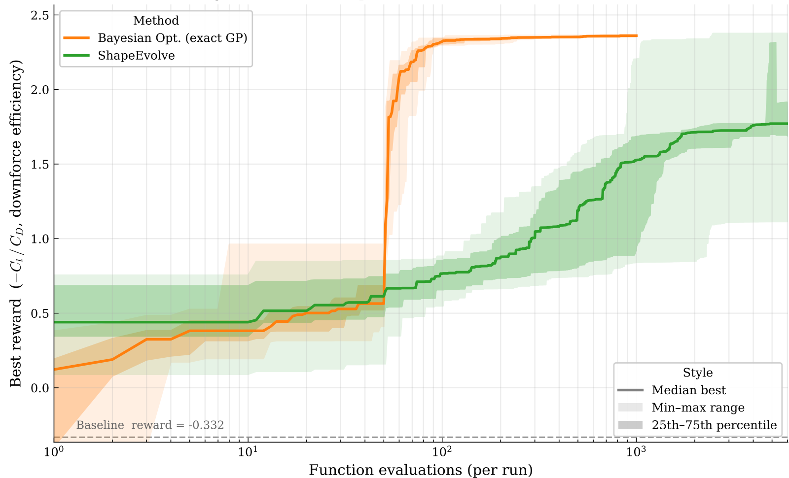
DrivAer * (Estate, vtk_E) — Downforce efficiency ( -C_l / C_D ) optimisation Convergence: best reward per run (solid = median, band = min-max)
