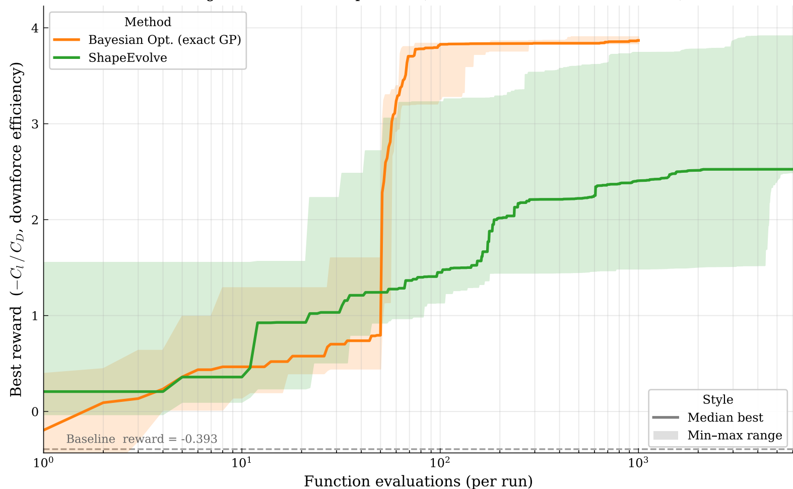
DrivAer * (Fastback, vtk_F) — Downforce efficiency ( -C_l/C_D ) optimisation Convergence: best reward per run (solid = median, band = min-max)
