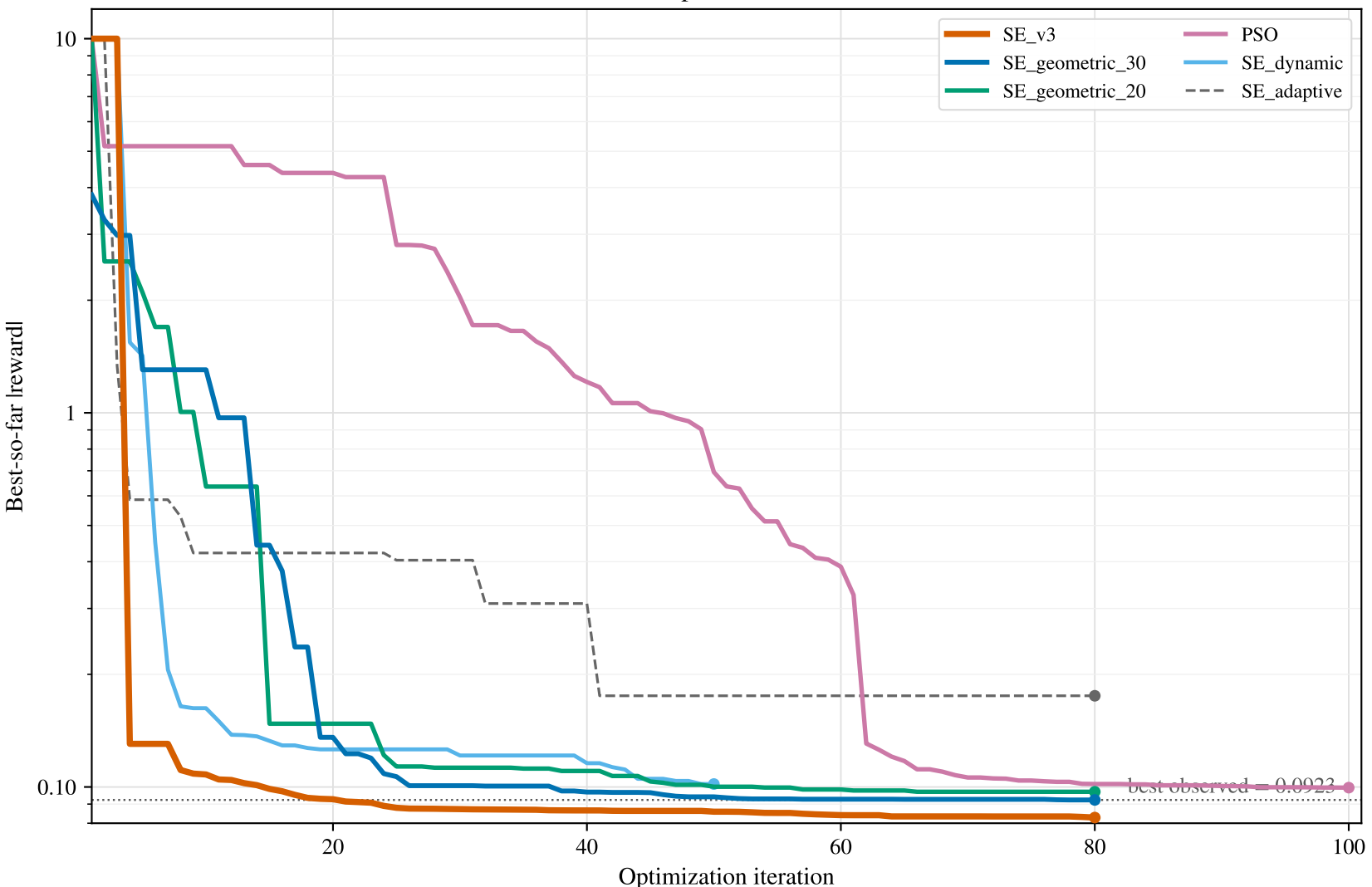
NeuralFoil Optimization Ablations
