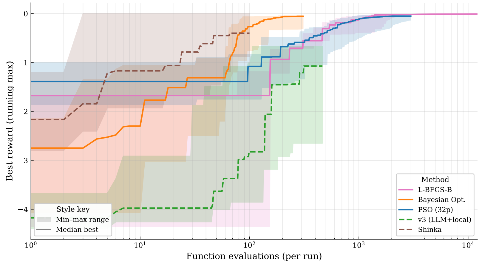
sw_005 — Minimise C_D (soft C_L floor)
