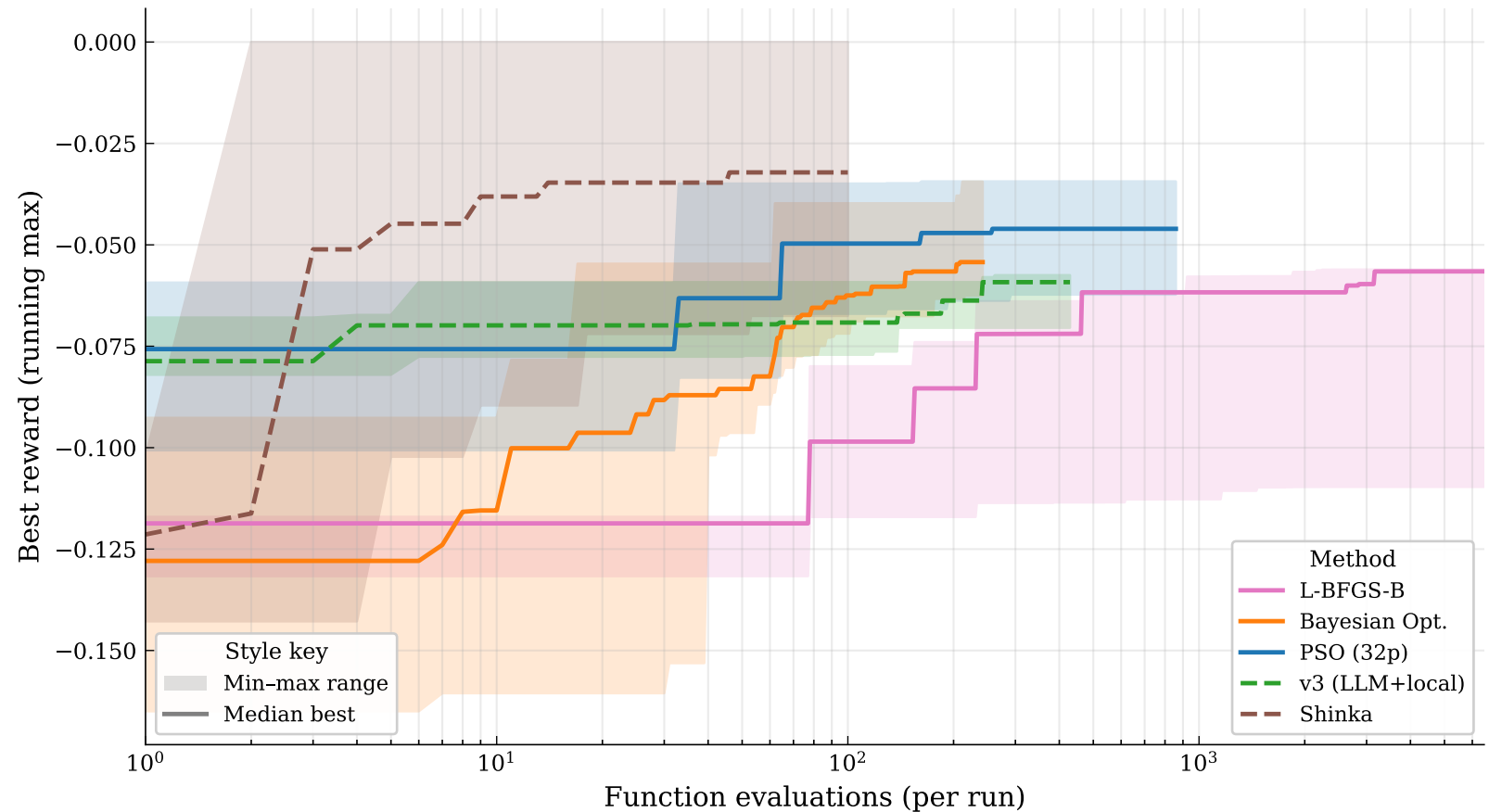
sw_010 — Minimise C_D at C_L = 0.55
