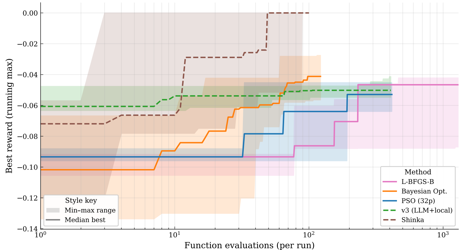
sw_015 — Minimise C_D (multi-point avg)
