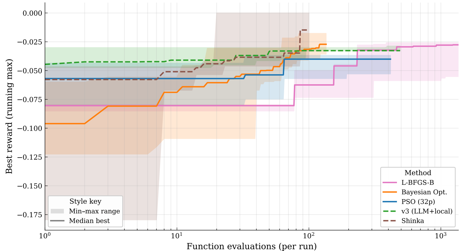
sw_016 — Minimise avg C_D across C_L targets
