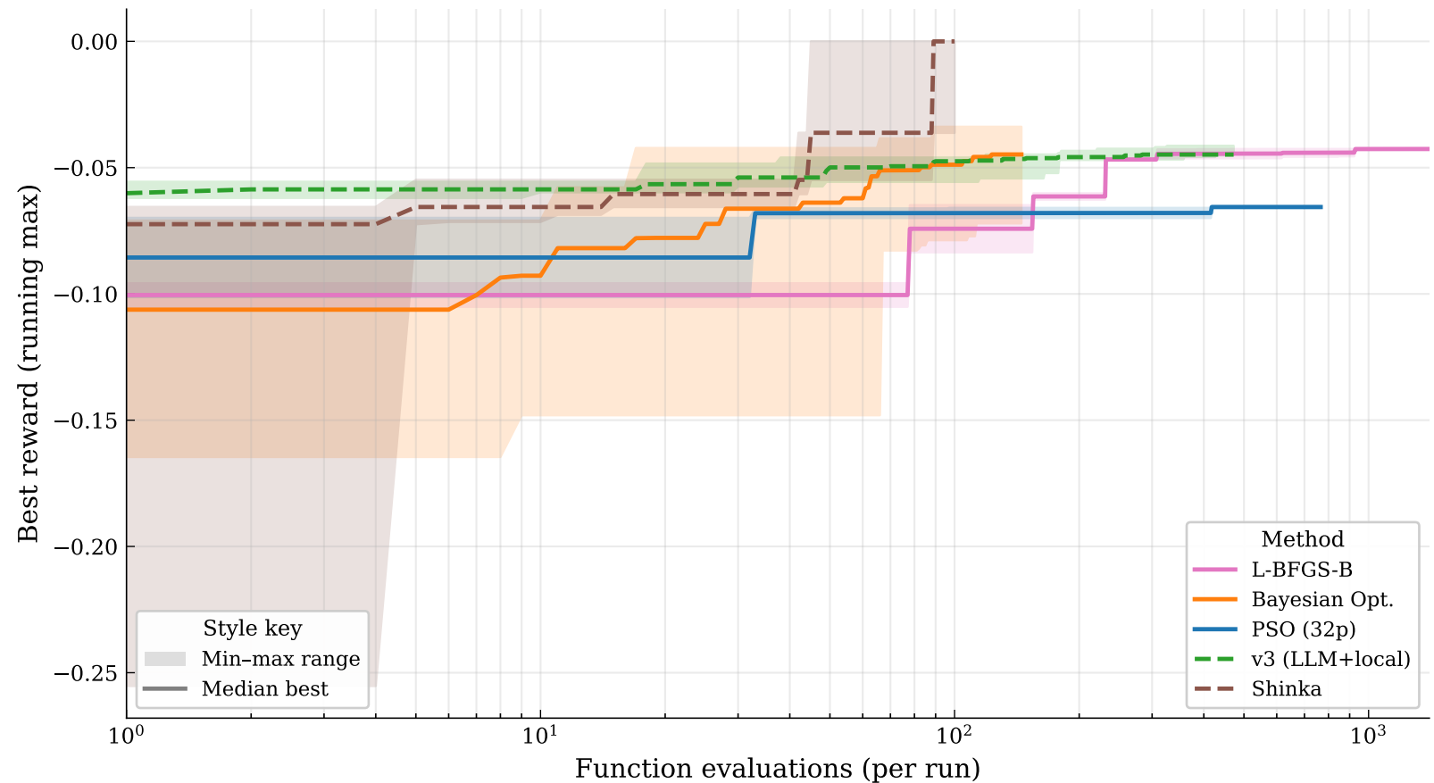
sw_018 — Minimise avg C_D across C_L targets
