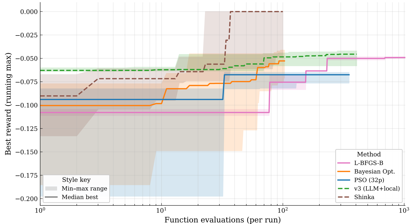
sw_020 — Minimise avg C_D across C_L targets
