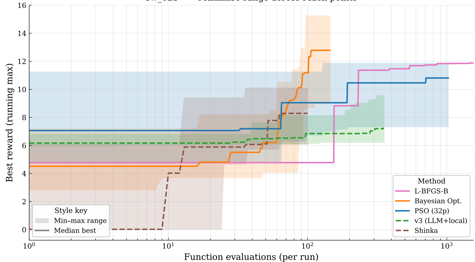
sw_023 — Maximise range across Mach points
