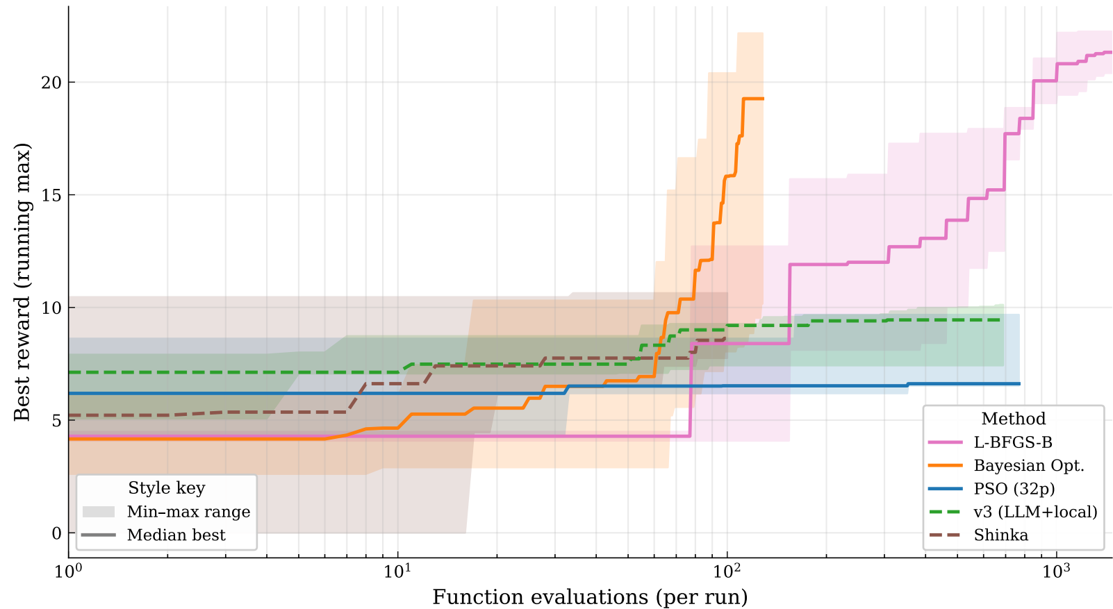
sw_028 — Maximise weighted range across C_L targets
