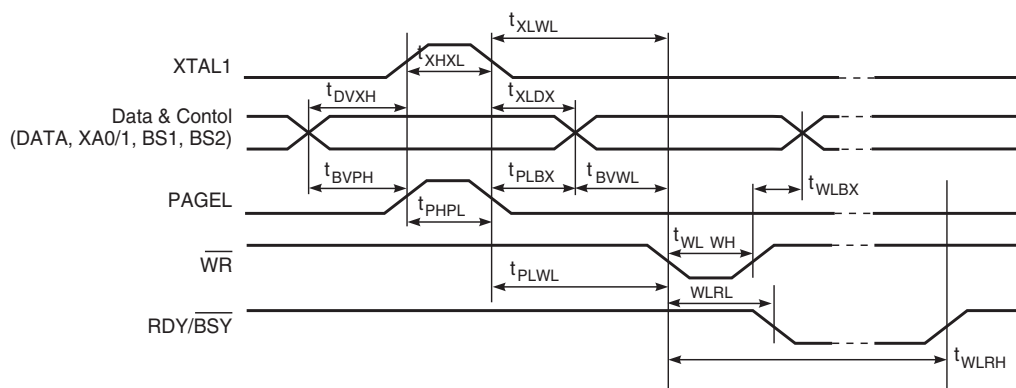
Figure 133. Parallel Programming Timing, Including some General Timing Requirements
