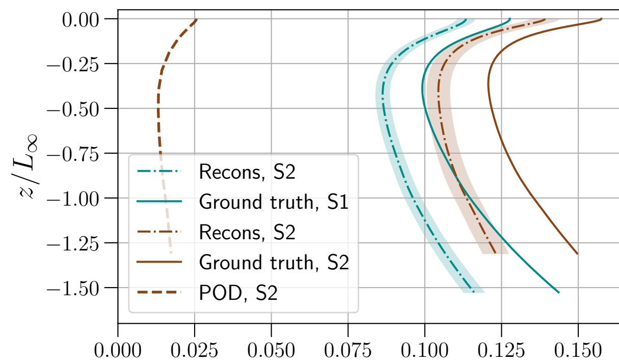
(a) \langle u_{RMS} \rangle , Cases S1 & S2
