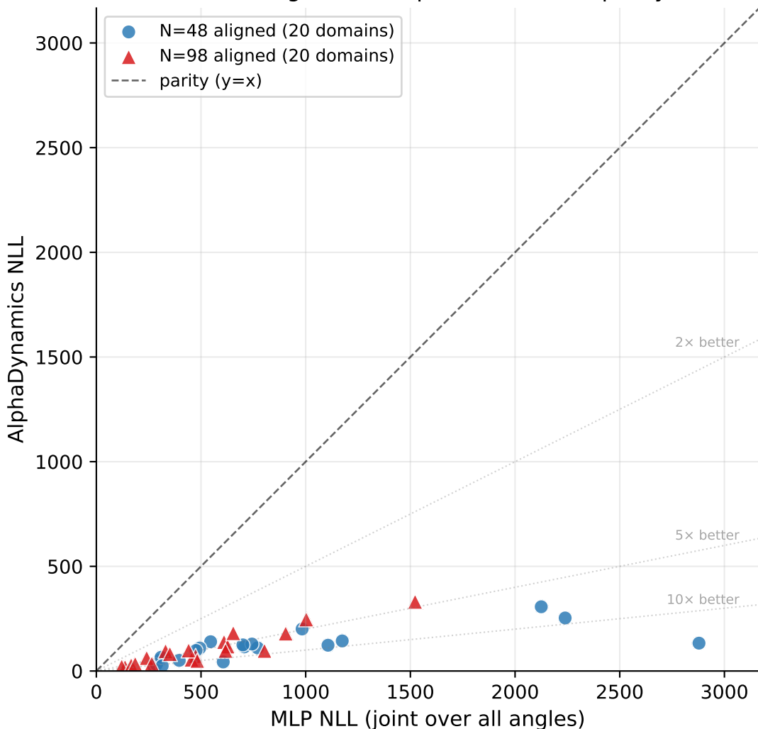
Per-domain NLL: AlphaDynamics vs MLP baseline 40/40 aligned audit points lie below parity
