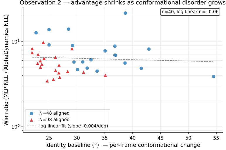
Figure 2: Observation 2: win ratio \text{NLL}_{\text{MLP}}/\text{NLL}_{\text{AlphaDynamics}} versus per-domain identity baseline. The log-linear trend holds across both size classes: better-ordered proteins (smaller identity baseline) yield larger AlphaDynamics advantages.
