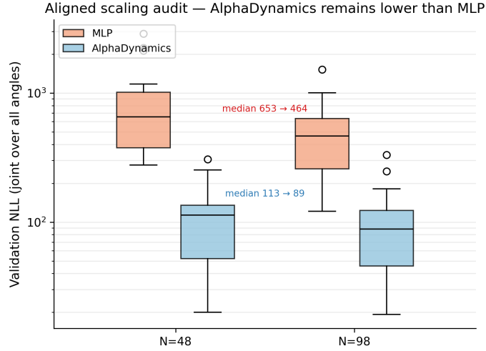
Figure 3: Scaling behaviour from aligned N = 48 (20 domains) to aligned N = 98 (20 domains). AlphaDynamics remains below the MLP baseline in both aligned size classes; the ratio is not monotonic with chain length after the alignment audit.
