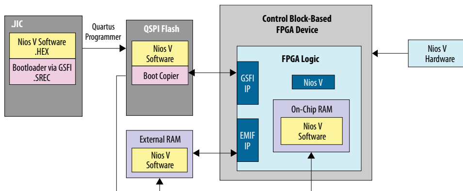
Figure 84. Nios V Processor Application Copied from General Purpose QSPI Flash to RAM Using Boot Copier (Bootloader via GSFI)
