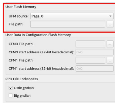
Figure 49. Setting Page_0 for UFM Source if Initialize Flash Content is Checked
