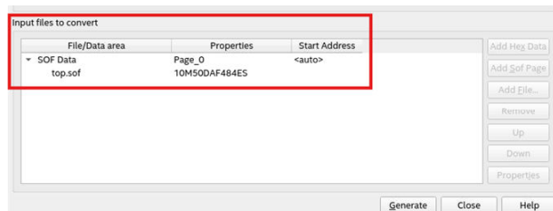
Figure 51. Input Files to Convert in Convert Programming Files for Single Image Mode
