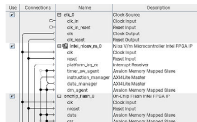
Figure 32. Connection between On-chip Flash IP and Nios V Processor
