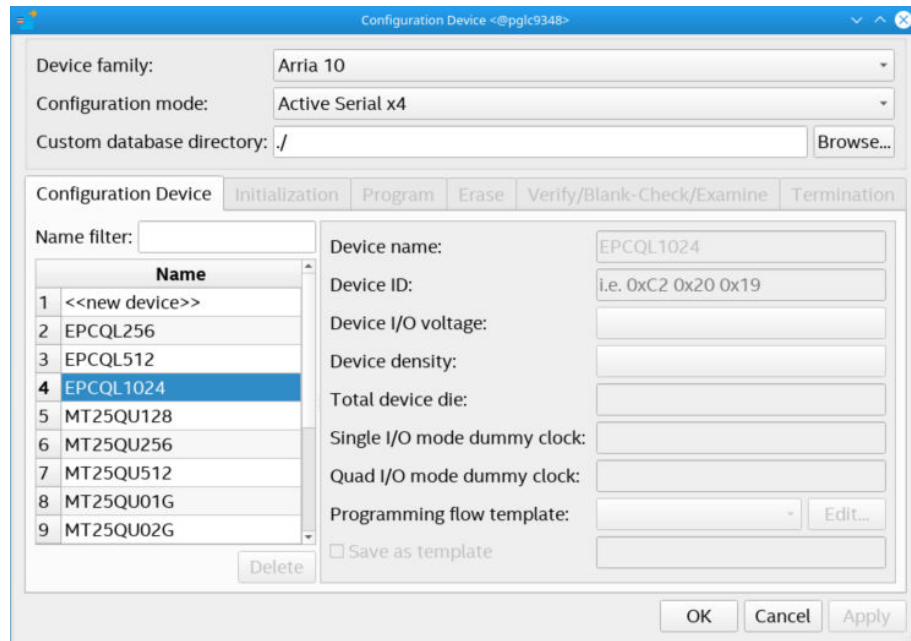
Figure 110. Configuration Device Window
