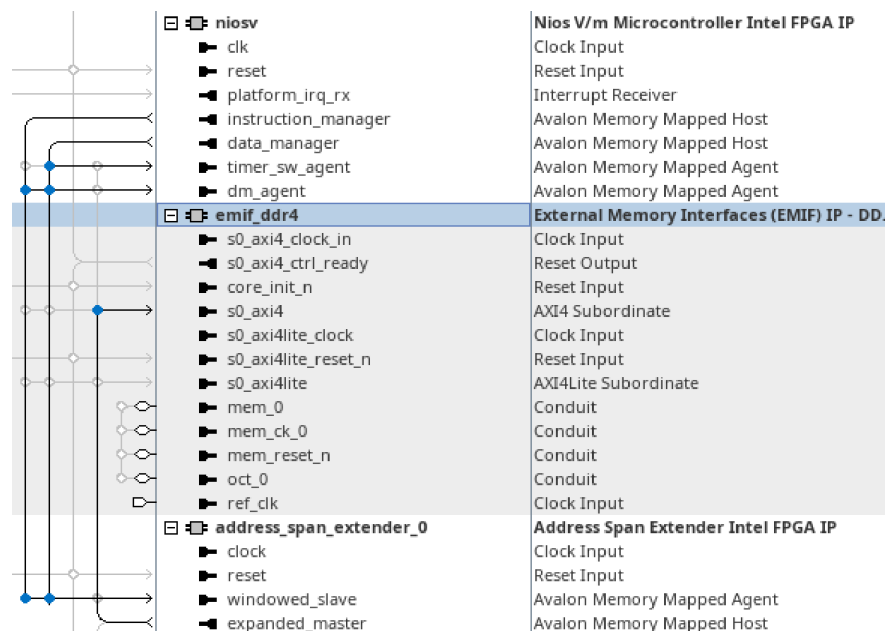
Figure 14. Connecting Instruction and Data Manager to Address Span Extender
