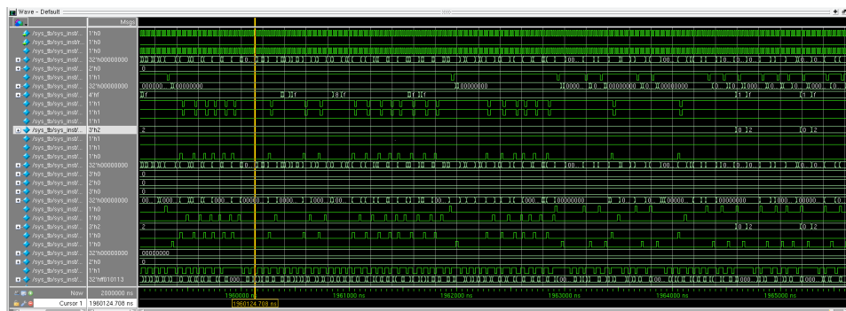
Figure 198. Simulation Result
