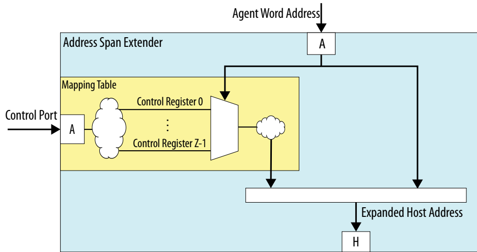
Figure 13. Address Span Extender Altera FPGA IP
