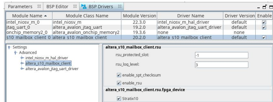
Figure 210. BSP Drivers Tab
