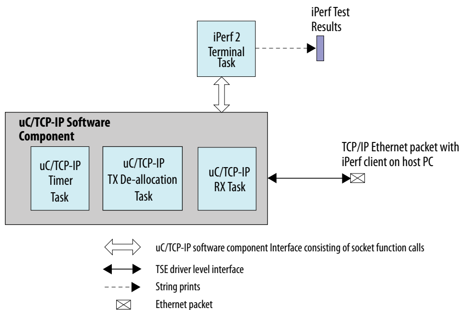
Figure 172. \mu C/TCP-IP IPerf Data Flow Diagram
