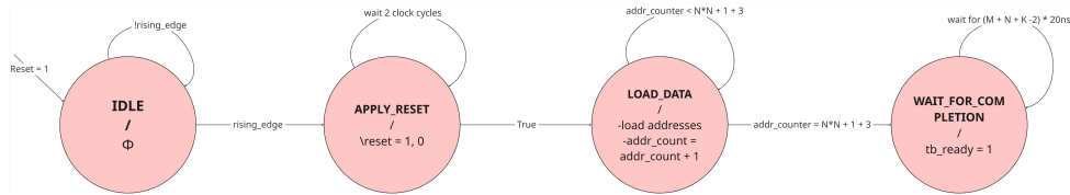
Figure 7 Testbench Finite State Machine (FSM) Diagram
