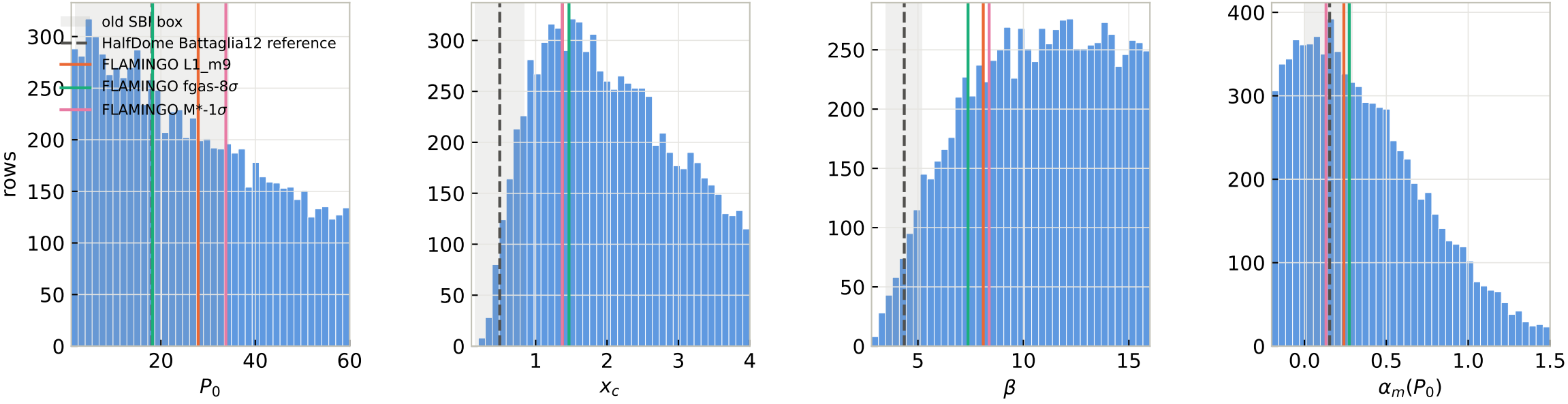
Accepted design marginals (linear-uniform base on the joint support), reference fits, and run statistics
