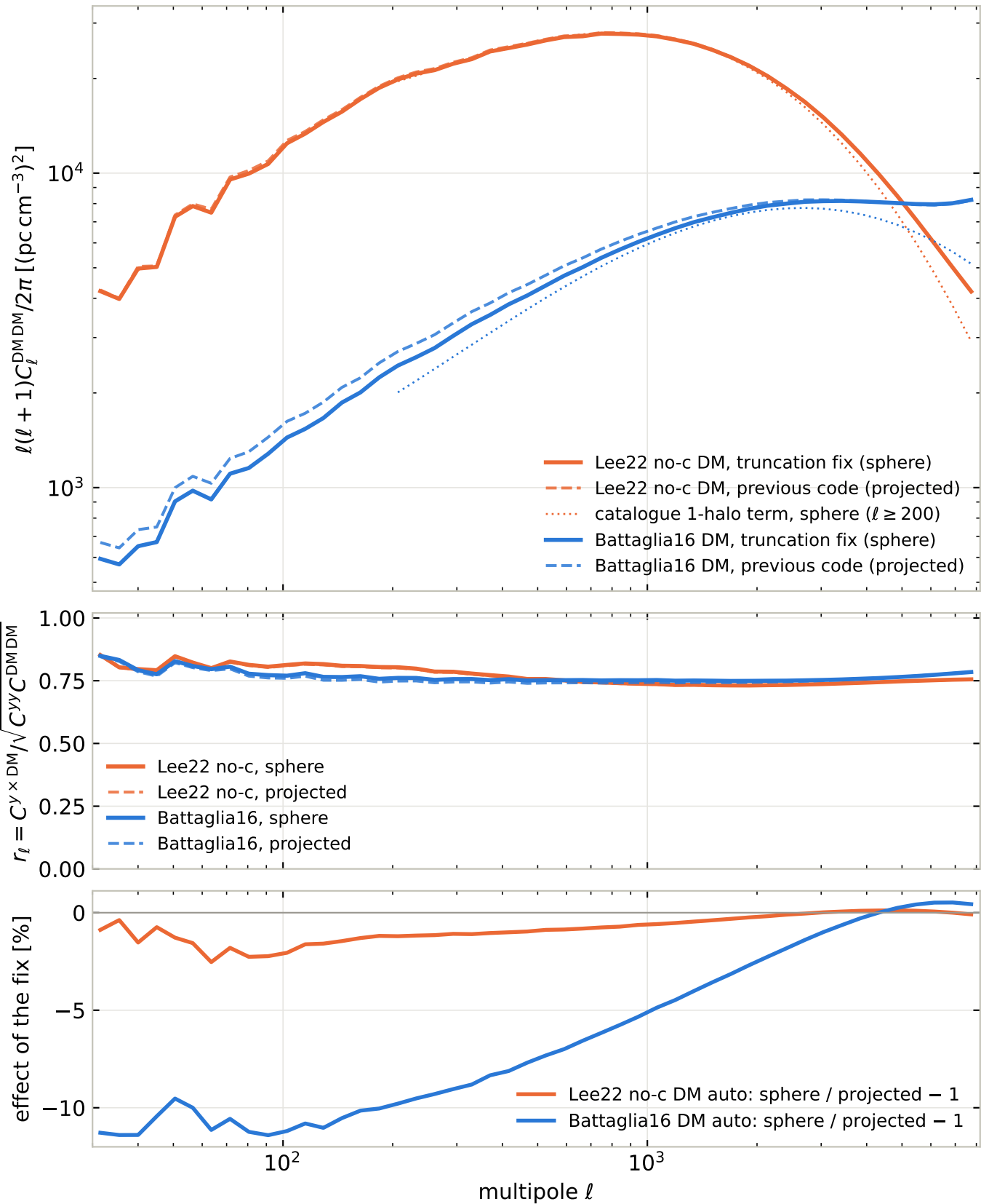
Halo-DM auto-spectra and correlation with y : Lee22 no-c vs Battaglia16, 4R_{200c}
