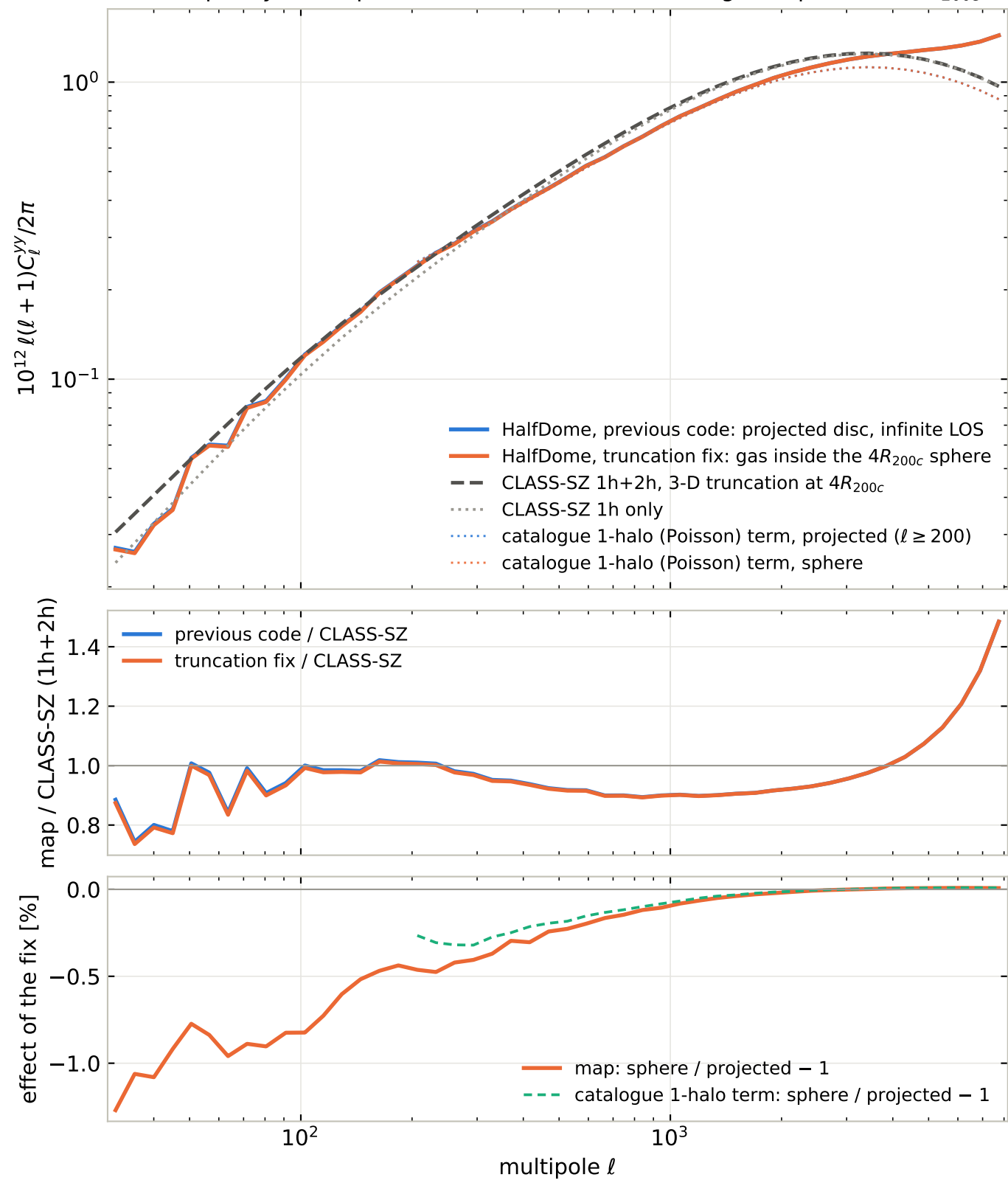
tSZ Compton-y auto-spectrum, HalfDome halos, Battaglia12 pressure, 4R_{200c}
