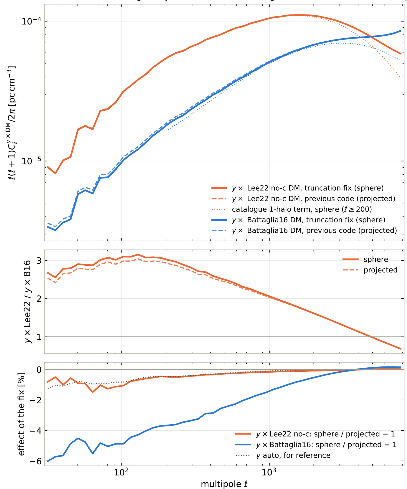
tSZ \times halo DM: Battaglia12 y \times Lee22 no-c vs Battaglia16 DM, HalfDome halos, 4R_{200c}
