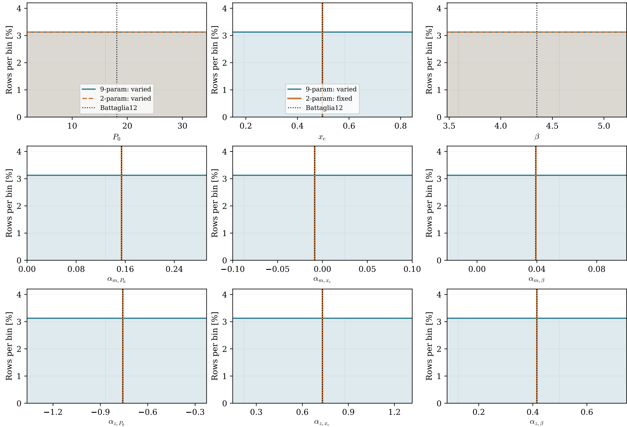
Actual Sobol parameter distributions: 32,768 rows per design 32 equal-width bins; uniform varied parameters give 3.125% per bin
