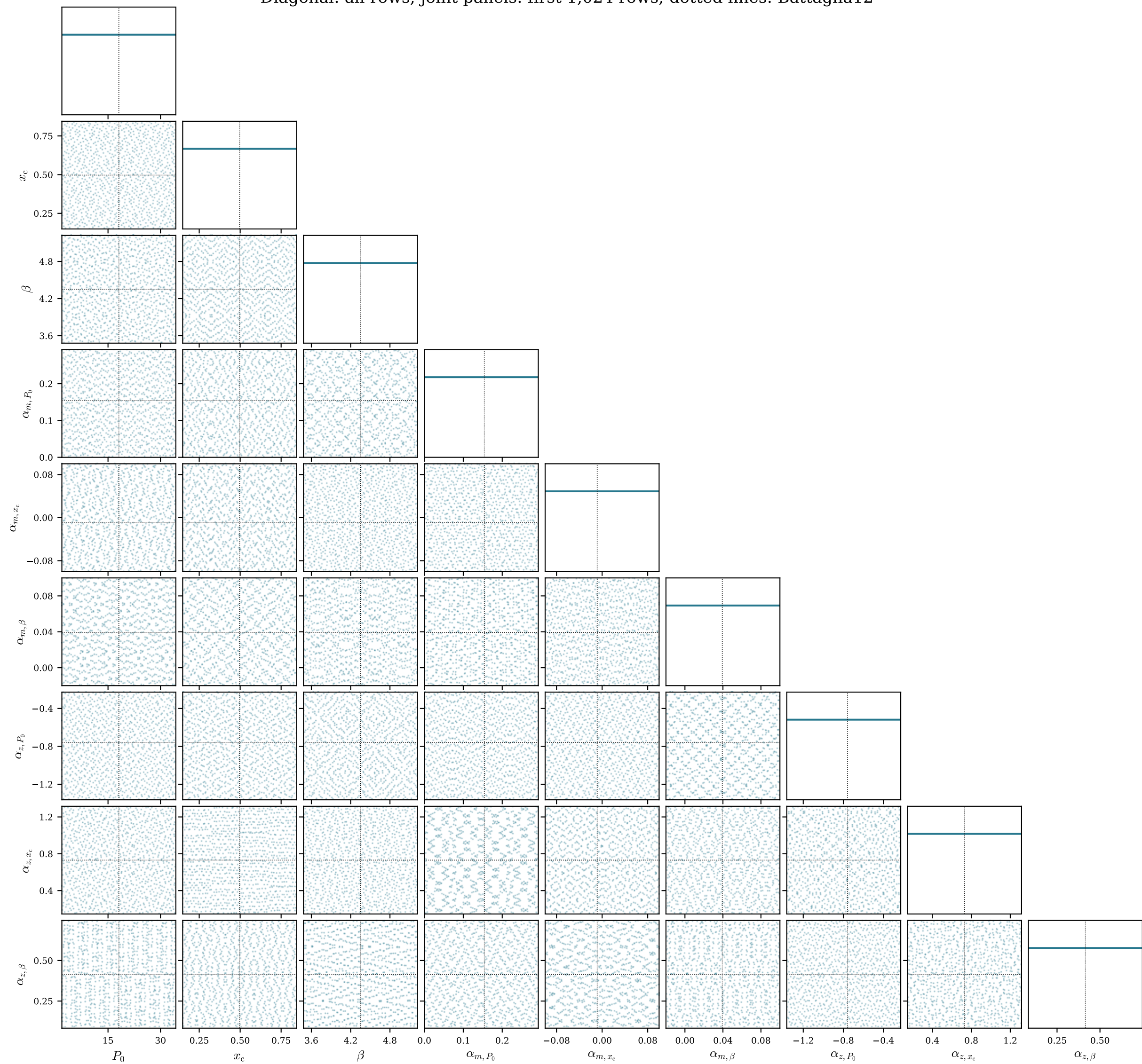
9-parameter Sobol design: N=32,768 (not posterior constraints) Diagonal: all rows; joint panels: first 1,024 rows; dotted lines: Battaglia12
