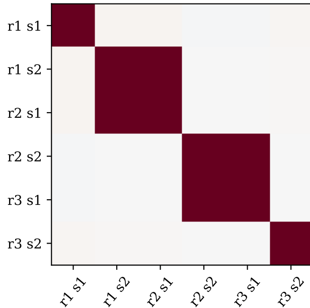
Stride 1: adjacent splits duplicate
