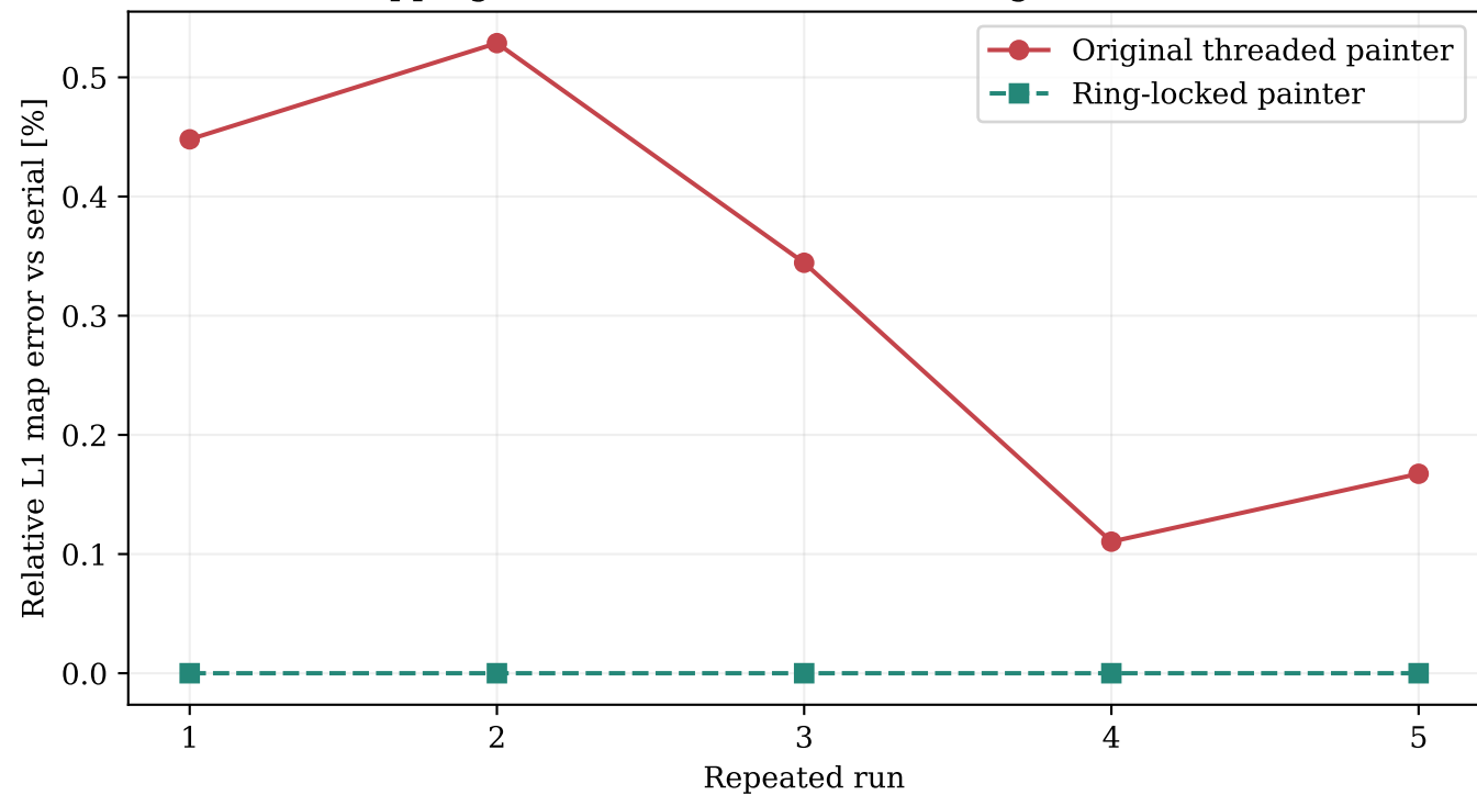
Overlapping-halo stress test (not a catalogue bias estimate)
